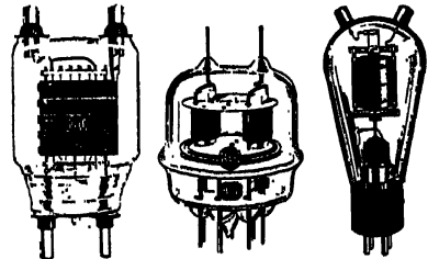
Transmitting tubes.
